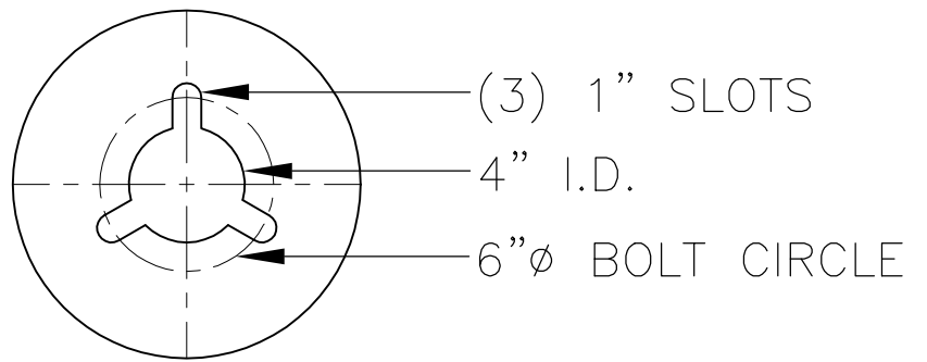
BASE DETAIL
