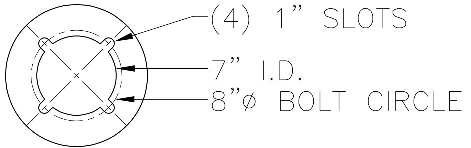
BASE DETAIL
