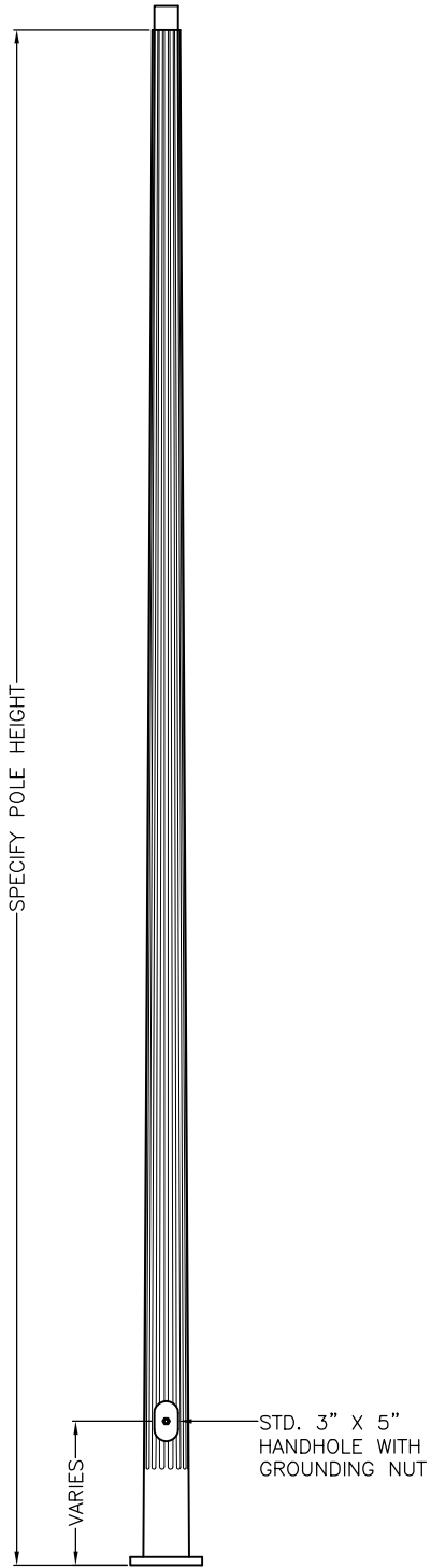
5 3/4" O.D. POLE
