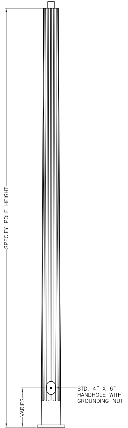
9" O.D. POLE
