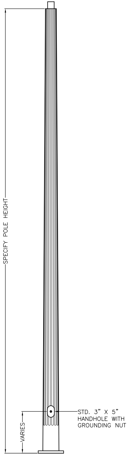
7" O.D. POLE
