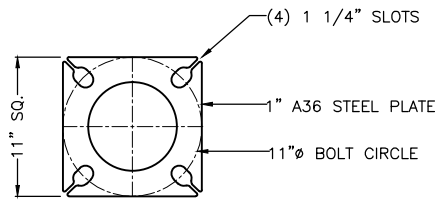
BASE PLATE DETAIL SCALE: 2X
