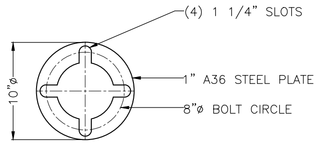
BASE PLATE DETAIL SCALE: 2X
