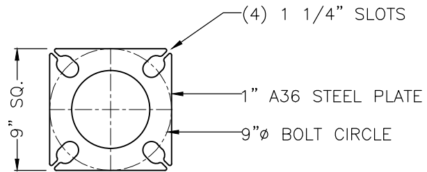
BASE PLATE DETAIL SCALE: 2X
