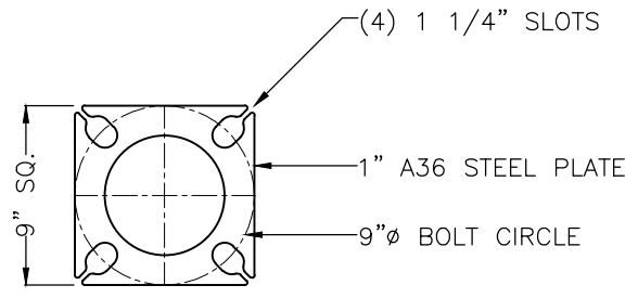
BASE PLATE DETAIL SCALE: 2X
