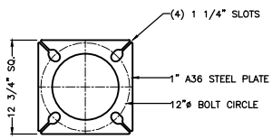
BASE PLATE DETAIL SCALE: 2X
