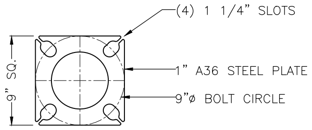
BASE PLATE DETAIL SCALE: 2X
