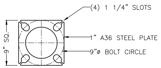
BASE PLATE DETAIL SCALE: 2X
