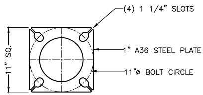
BASE PLATE DETAIL SCALE: 2X
