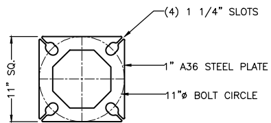
BASE PLATE DETAIL SCALE: 2X
