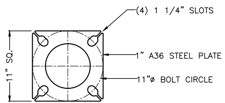
BASE PLATE DETAIL SCALE: 2X
