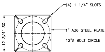
BASE PLATE DETAIL SCALE: 2X
