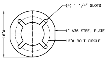
BASE PLATE DETAIL SCALE: 2X
