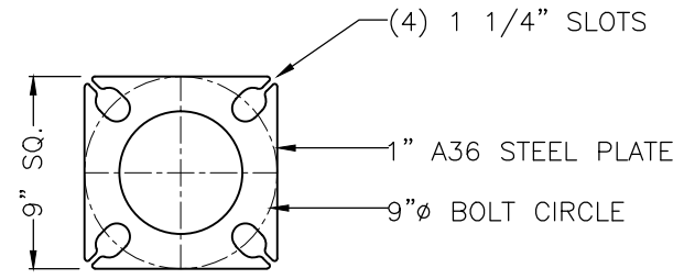
BASE PLATE DETAIL SCALE: 2X
