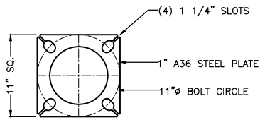
BASE PLATE DETAIL SCALE: 2X
