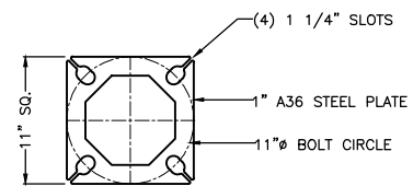
BASE PLATE DETAIL SCALE: 2X
