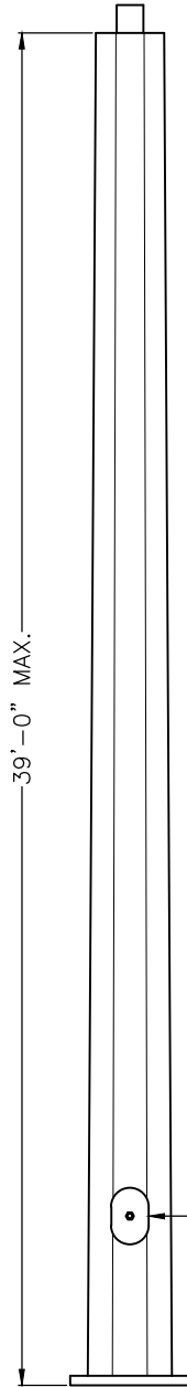
9" FLAT-TO-FLAT POLE
