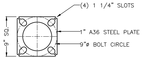
BASE PLATE DETAIL SCALE: 2X
