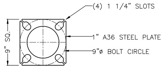
BASE PLATE DETAIL SCALE: 2X
