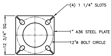
BASE PLATE DETAIL SCALE: 2X
