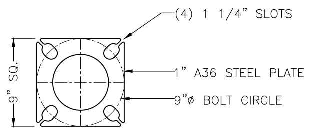
BASE PLATE DETAIL SCALE: 2X
