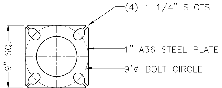
BASE PLATE DETAIL
