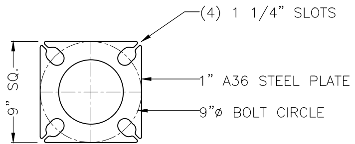
BASE PLATE DETAIL SCALE: 2X
