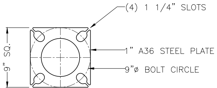
BASE PLATE DETAIL
