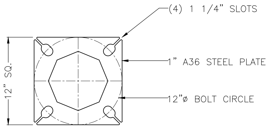
BASE PLATE DETAIL SCALE: 2X
