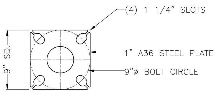
BASE PLATE DETAIL SCALE: 2X
